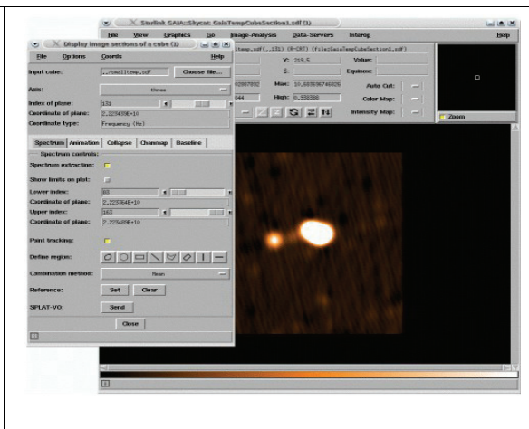
Figure 38. Snapshot of GAIA SkyCat application.
