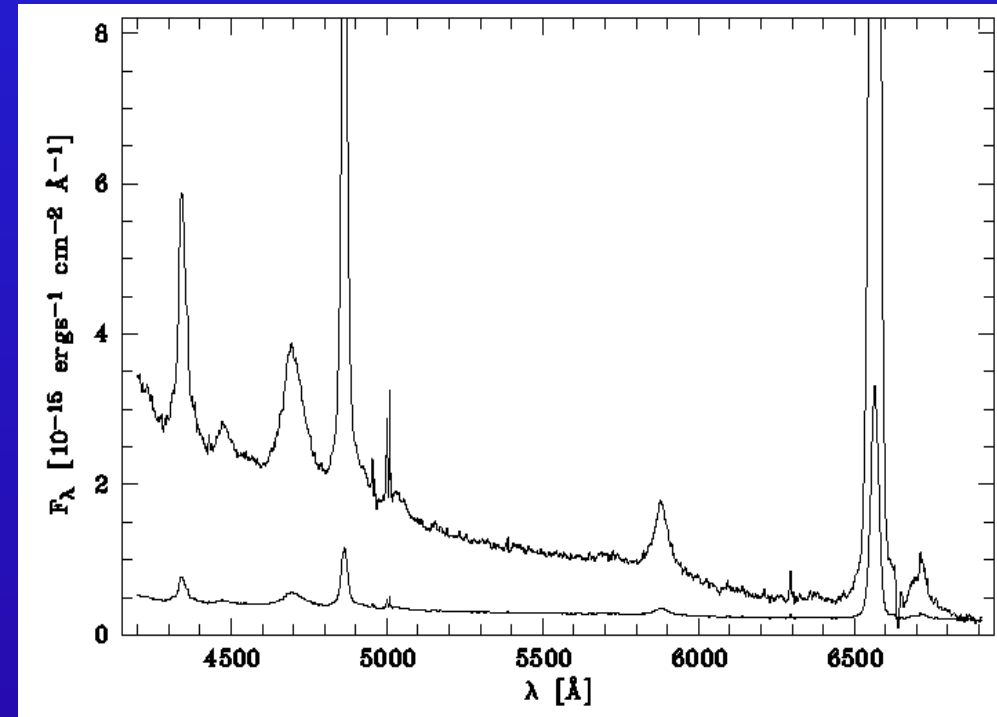
Rms spectrum
