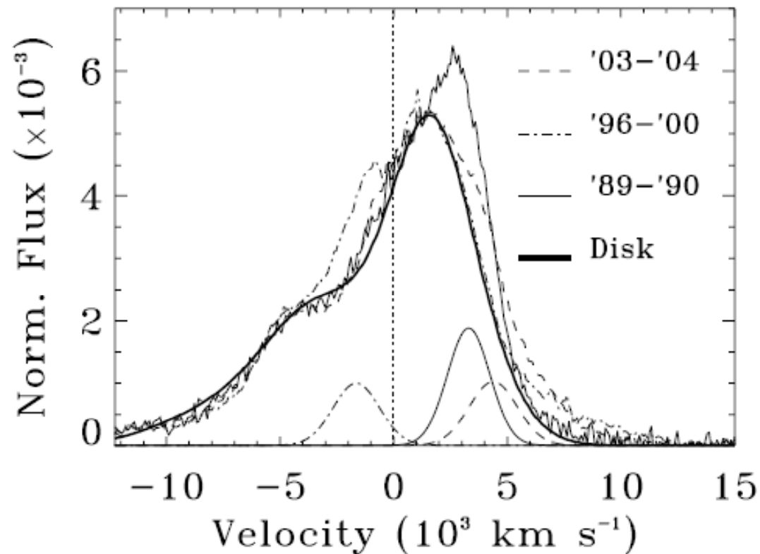
FIG. 30.—Mrk 668: Averaged broad H \alpha profiles that demonstrate the dramatic changes in the red central peak. The thick solid line shows the eccentric disk fit to the nonvarying portion of the profile. The variations in the profile are modeled with Gaussian excesses superposed on the eccentric disk profile that drift from the red side to the blue side of the profile and back. These are shown at the bottom of the figure, following the line style convention of the legend. See also the discussion in § 4.5.3.
